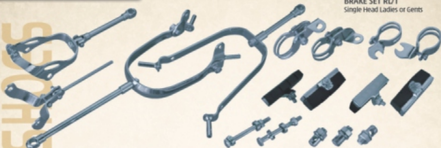
SE-601-P BRAKE SET PH/T Single or Double Head Ladies or Gents
